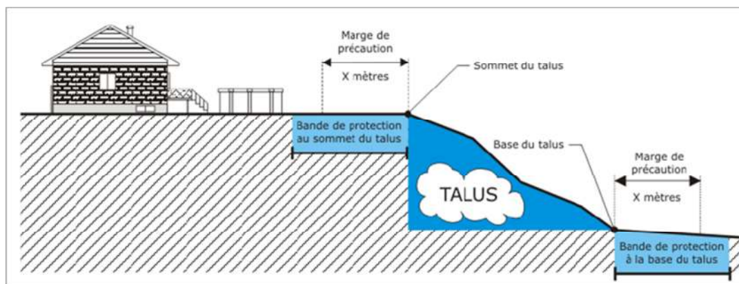
Figure 6.1 - Talus
